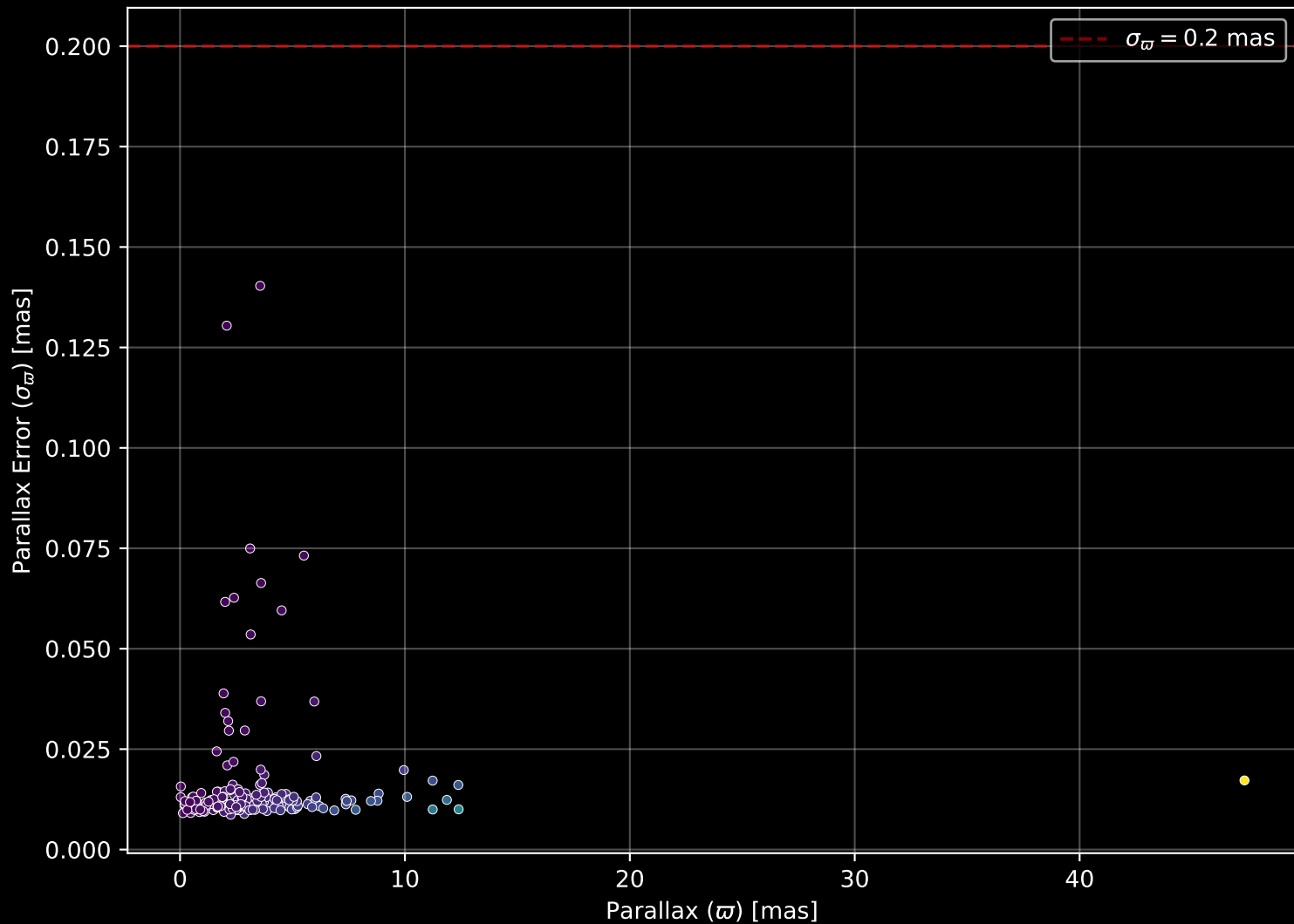
APOGEE DR17 Field: [065+48_MGA] Parallax Quality (n= 197)
