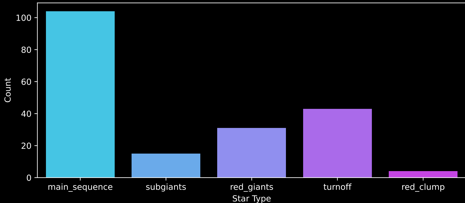
APOGEE DR17 Field: [065+48_MGA] Count plot of Star Type
