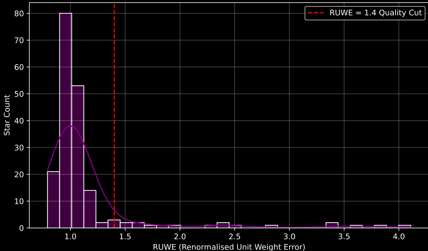
GAPOGEE DR17 Field [065+48_MGA] RUWE Distribution (n= 190)
