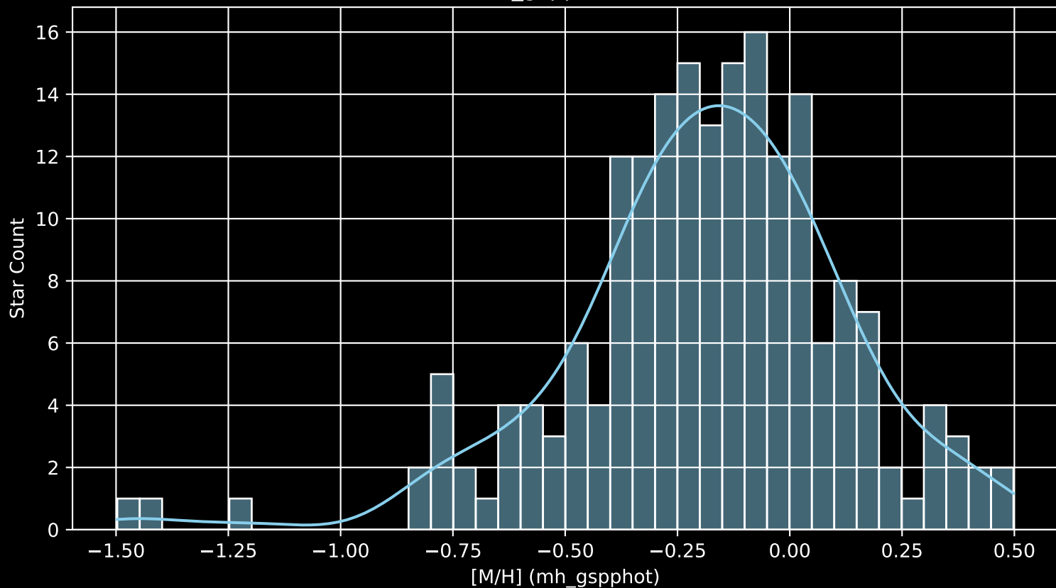
APOGEE DR17 Field: [065+48_MGA [M/H] (mh_gspphot) (n= 192)
