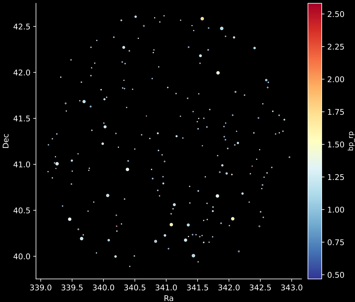
APOGEE DR17 Field: [065+48_MGA] Stars: 197
