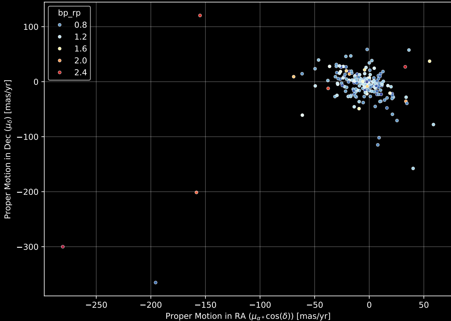
APOGEE DR17 Field: [065+48_MGA] Proper Motion Diagram (n= 197)
