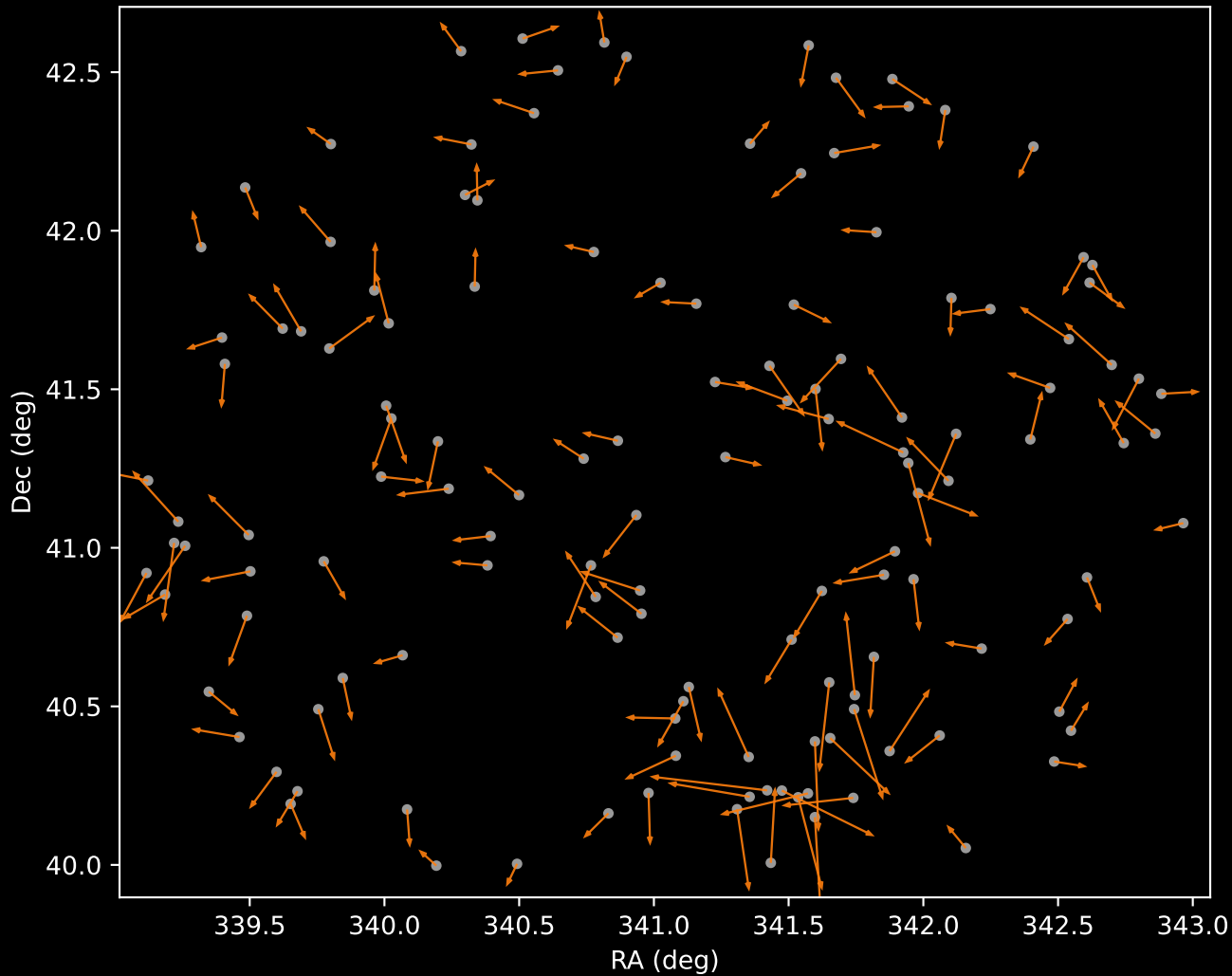
APOGEE DR17 Cluster 2 Proper Motion Vectors (n=135)
